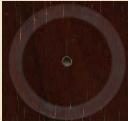
海島型地板 (4,000轉) : 表層已磨穿並龜裂 Engineered flooring (4,000 turns) : Surface has been grinded and cracked
