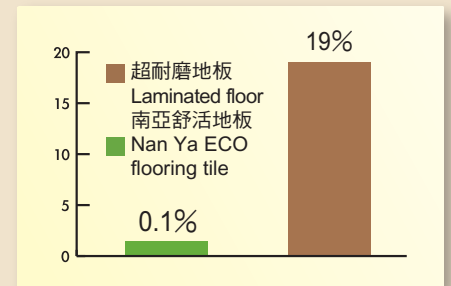
吸水厚度膨脹變化率 (%) Thickness swelling changing rate of water absorption (%)
